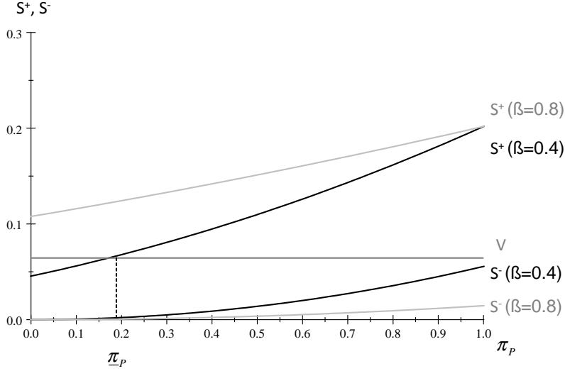
Figure 6: Surplus from trade with exogenous \beta
