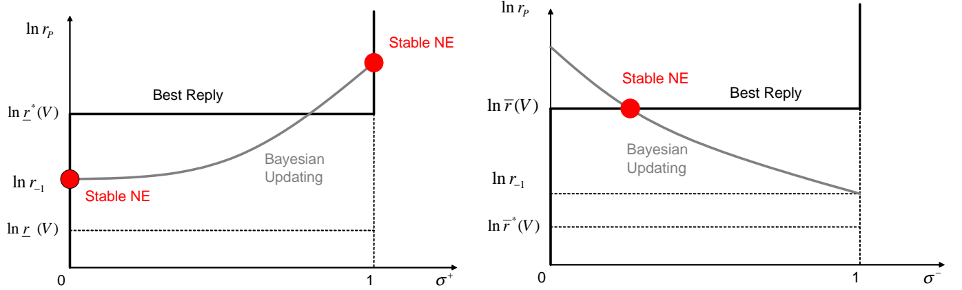
Figure 7: Multiple PBE and Mixed-Strategy PBE
